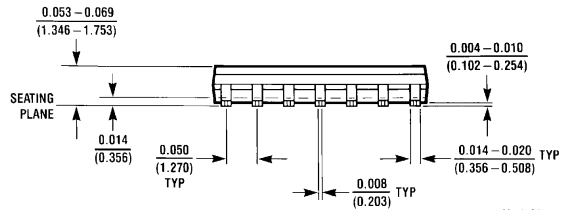
14-Lead Small Outline Molded Package (M) Order Number DM74LS55M NS Package Number M14A
